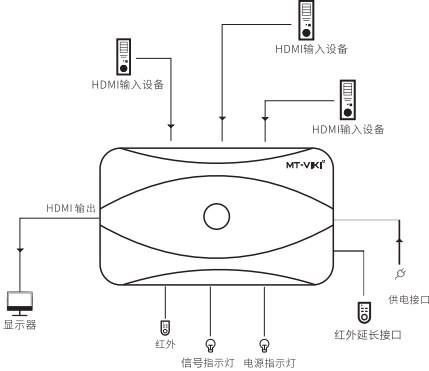
MT-HD0301
