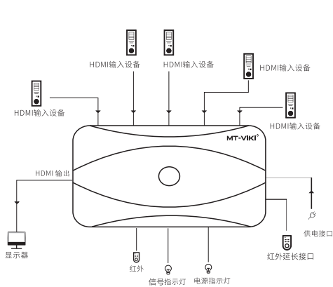
MT-HD0501
